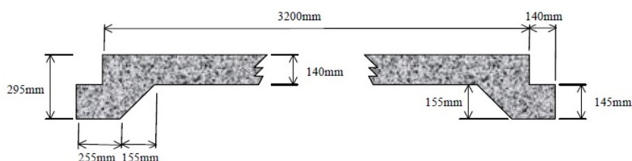
Figure 3.1: Floor/ceiling system
